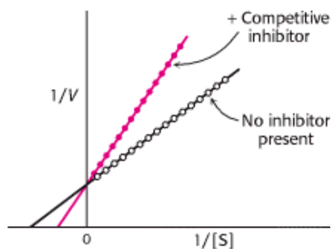
Figure 8.37. Competitive Inhibition Illustrated on a Double-Reciprocal Plot. A double-reciprocal plot of enzyme kinetics in the presence ( \text{---}\bullet\text{---} ) and absence ( \text{---}\circ\text{---} ) of a competitive inhibitor illustrates that the inhibitor has no effect on V_{\max} but increases K_M .
