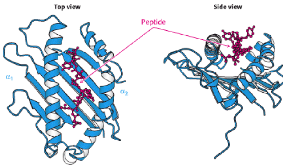
Figure 33.24. Class I MHC Peptide-Binding Site. The α 1 and α 2 domains come together to form a groove in which peptides are displayed. The two views shown reveal that the peptide is surrounded on three sides by a β sheet and two α helices, but it is accessible from the top of the structure.
