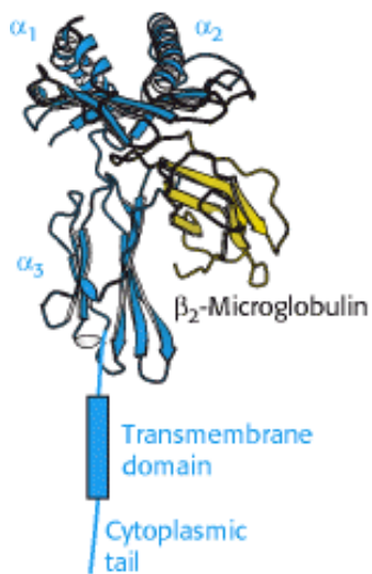
Figure 33.23. Class I MHC Protein. A protein of this class consists of two chains. The α chain begins with two domains that include α helices (α 1 , α 2 ), an immunoglobulin domain (α 3 ), a transmembrane domain, and a cytoplasmic tail. The second chain, β 2 -microglobulin, adopts an immunoglobulin fold.
