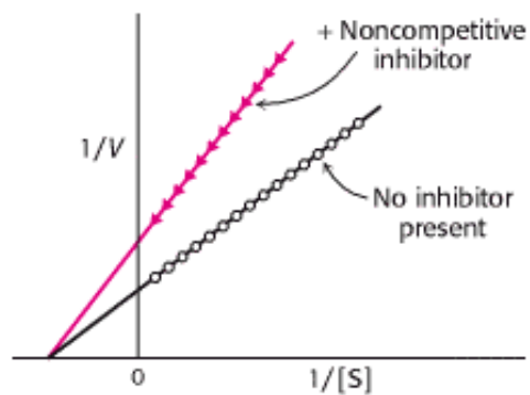
Figure 8.38. Noncompetitive Inhibition Illustrated on a Double-Reciprocal Plot. A double-reciprocal plot of enzyme kinetics in the presence ( \text{---}\bullet\text{---} ) and absence ( \text{---}\circ\text{---} ) of a noncompetitive inhibitor shows that K_M is unaltered and V_{\max} is decreased.
