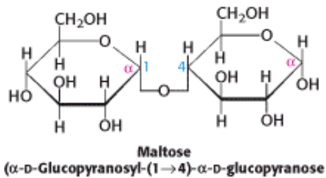
Figure 11.11. Common Disaccharides. Sucrose, lactose, and maltose are common dietary components.
