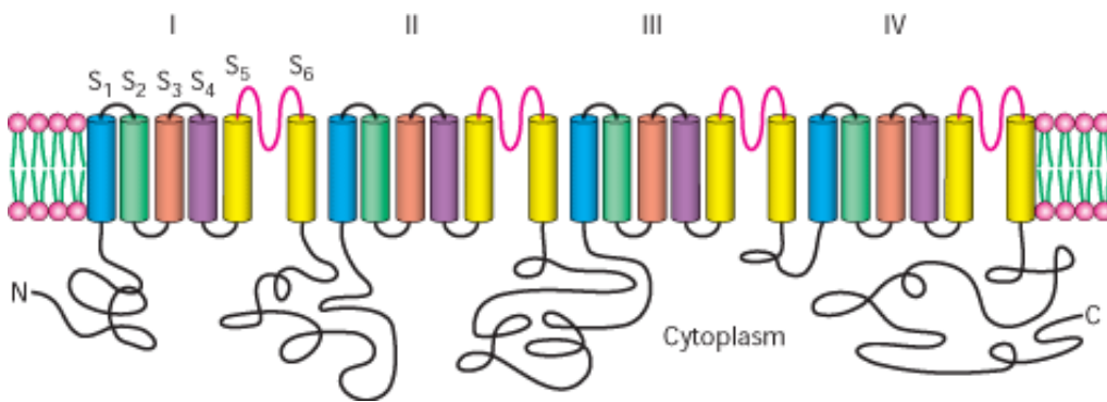
Figure 13.20. The Sodium Channel. The Na + channel is a single polypeptide chain with four repeating units (I–IV). Each repeat probably folds into six transmembrane helices. The loops (shown in red) between helices 5 and 6 of each domain form the pore of the channel.
