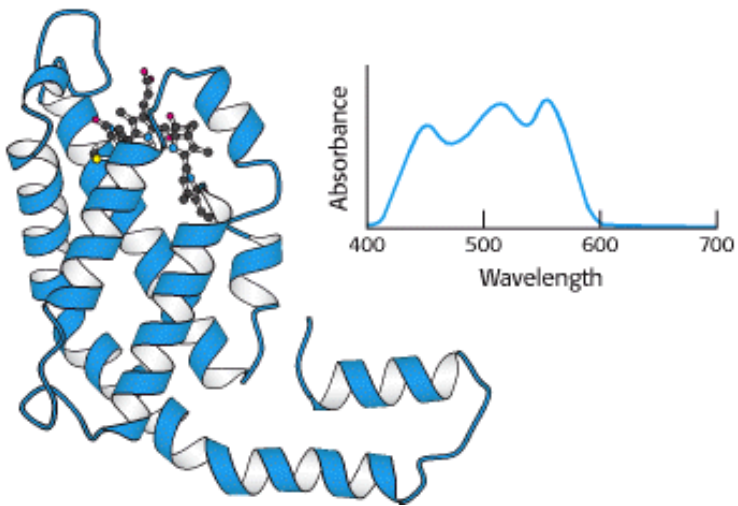
Figure 19.31. Structure of a Phycobilisome Subunit. This protein, a phycocerythrin, contains a phycocerythrobilin linked to a cysteine residue. The inset shows the absorption spectrum of a phycocerythrin.
