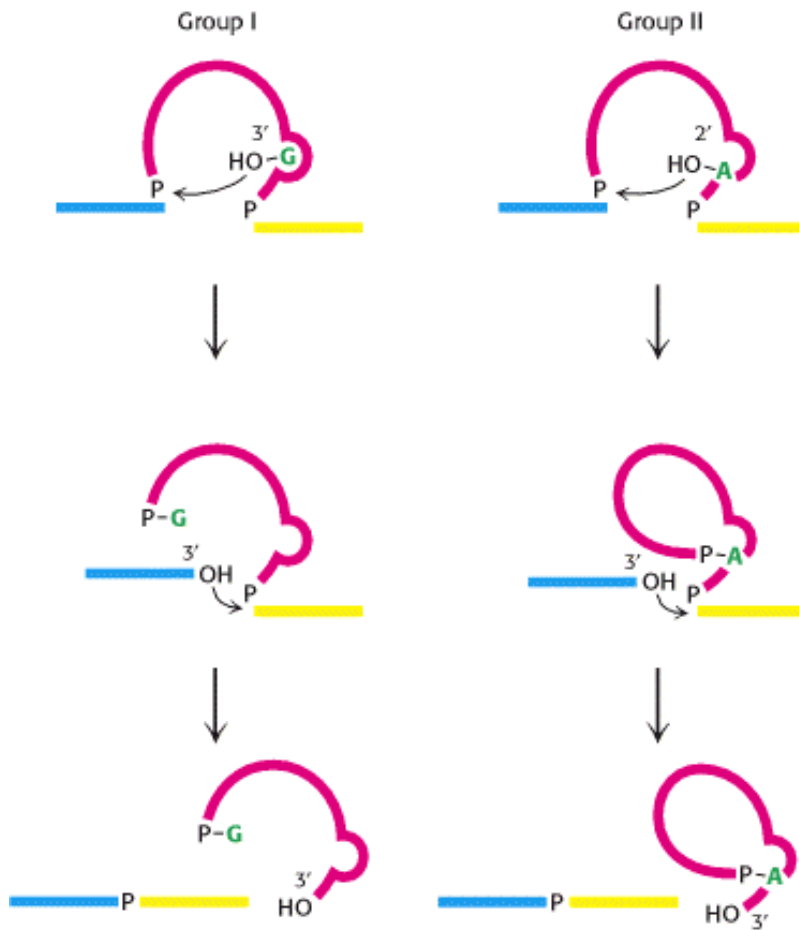
Figure 28.37. Comparison of Splicing Pathways. The exons being joined are shown in blue and yellow and the attacking unit is shown in green. The catalytic site is formed by the intron itself (red) in group I and group II splicing. In contrast, the splicing of nuclear mRNA precursors is catalyzed by snRNAs and their associated proteins in the spliceosome. [After P. A. Sharp. Science 235(1987):769.]
