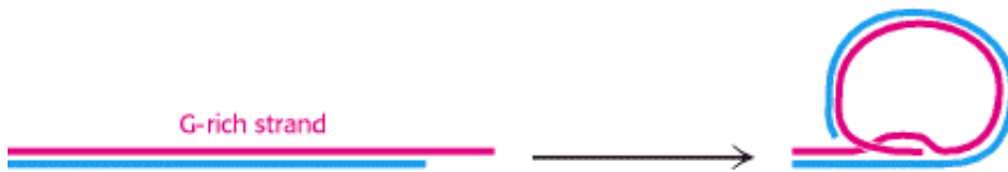
Figure 27.35. Proposed Model for Telomeres. A single-stranded segment of the G-rich strand extends from the end of the telomere. In one model for telomeres, this single-stranded region invades the duplex to form a large duplex loop.
