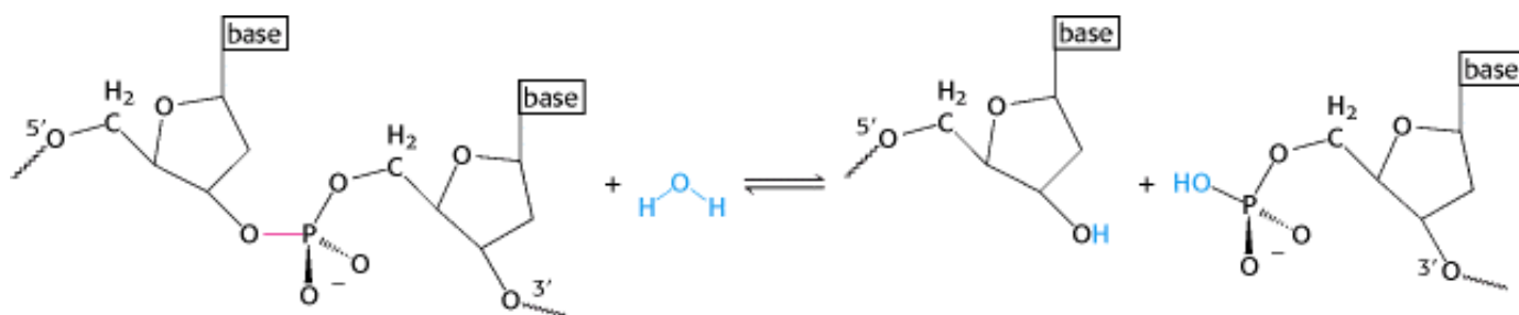
Figure 9.33. Hydrolysis of a Phosphodiester Bond. All restriction enzymes catalyze the hydrolysis of DNA phosphodiester bonds, leaving a phosphoryl group attached to the 5' end. The bond that is cleaved is shown in red.
