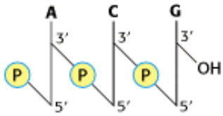
Figure 5.7. Structure of a DNA Chain. The chain has a 5 th end, which is usually attached to a phosphate, and a 3 rd end, which is usually a free hydroxyl group.
