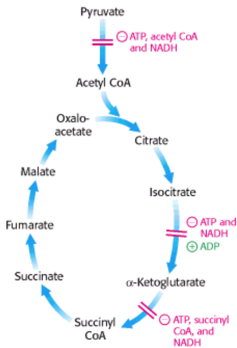
Figure 17.18. Control of the Citric Acid Cycle. The citric acid cycle is regulated primarily by the concentration of ATP and NADH. The key control points are the enzymes isocitrate dehydrogenase and α-ketoglutarate dehydrogenase.
