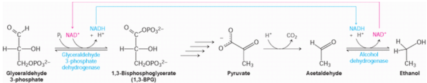
Figure 16.12. Maintaining Redox Balance. The NADH produced by the glyceraldehyde 3-phosphate dehydrogenase reaction must be reoxidized to NAD + for the glycolytic pathway to continue. In alcoholic fermentation, alcohol dehydrogenase oxidizes NADH and generates ethanol. In lactic acid fermentation (not shown), lactate dehydrogenase oxidizes NADH while generating lactic acid.
