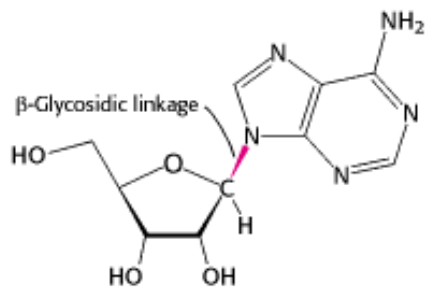
Figure 5.5. \beta -Glycosidic linkage in a nucleoside.
